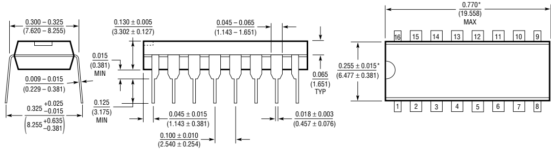
N Package 16-Lead Plastic DIP
