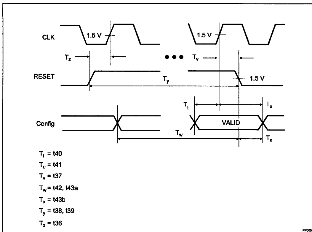
Figure 7. Reset and Configuration Timings
