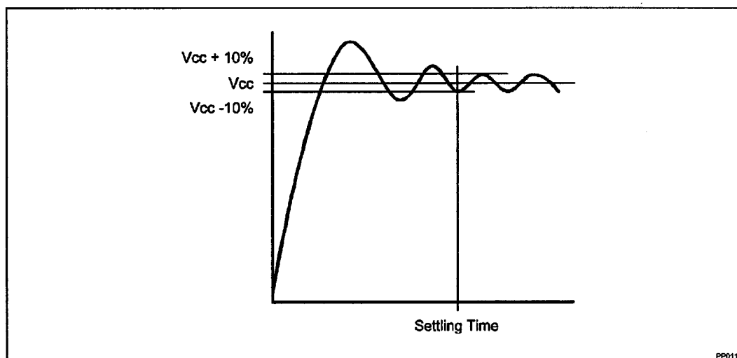
Figure 14. Settling Time
