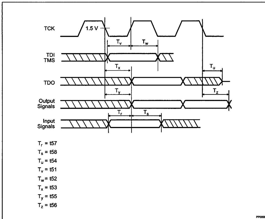
Figure 8. Test Timings
