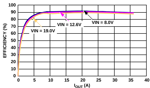
FIGURE 4. ACTIVE MODE EFFICIENCY, 2 PHASE, CCM, PSI_I = \text{HIGH} , VID = 1.15V
