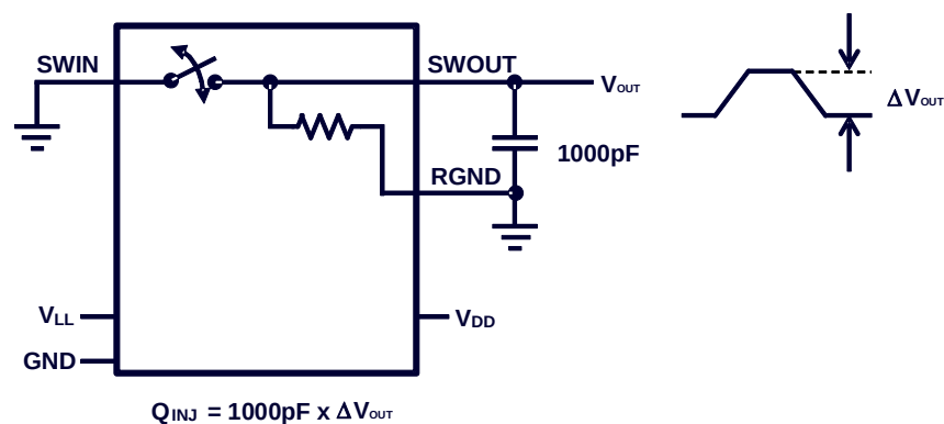
Figure 8: Test Circuit 7
