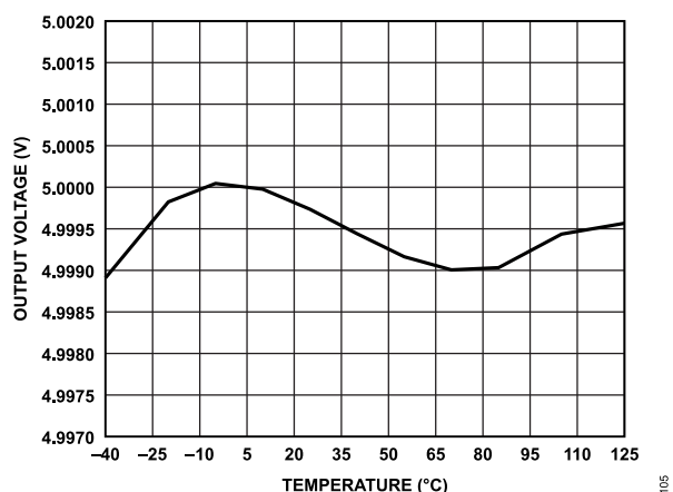
Figure 5. ADR3650 Output Voltage vs. Temperature
