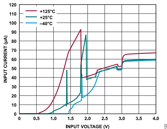
Figure 23. ADR3630 Input Current vs. Input Voltage
