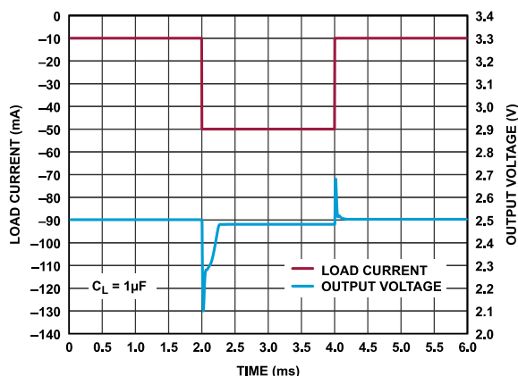
Figure 73. ADR3625 50 mA Sourcing Response
