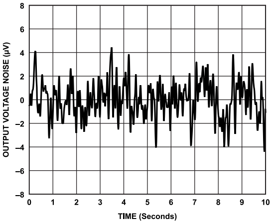
Figure 43. ADR3630 Voltage Noise (0.1 Hz to 10 Hz)
