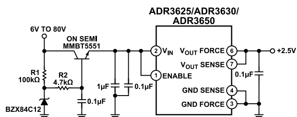
Figure 78. Extended Supply Range
