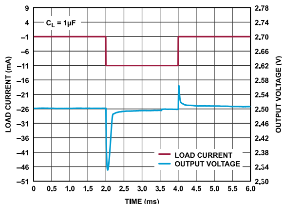
Figure 71. ADR3625 10 mA Sourcing Response
