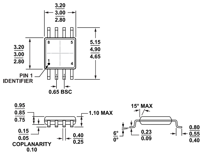
Figure 81. 8-Lead Mini Small Outline Package [MSOP] (RM-8) Dimensions shown in millimeters
