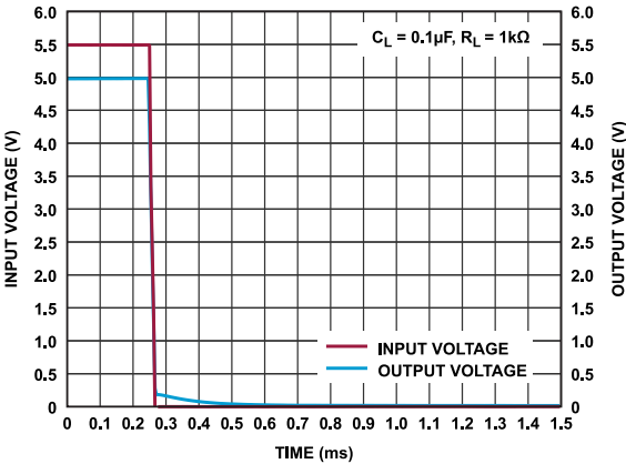
Figure 39. ADR3650 Shutdown Response (Input)
