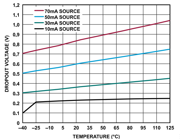
Figure 8. ADR3625 Dropout Voltage vs. Temperature
