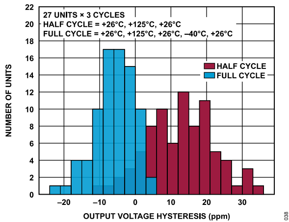
Figure 59. ADR3625 Hysteresis Histogram
