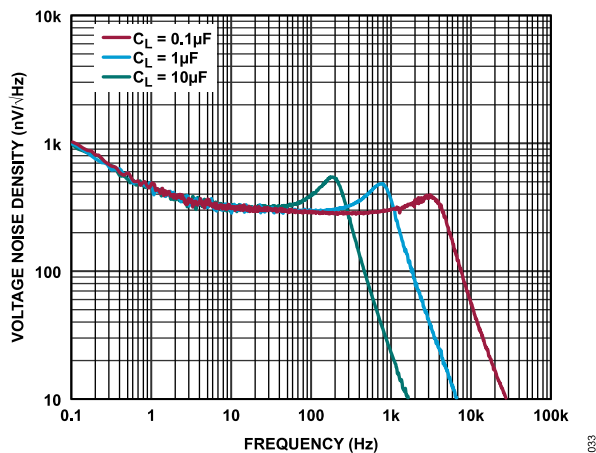
Figure 51. ADR3625 Voltage Noise Density
