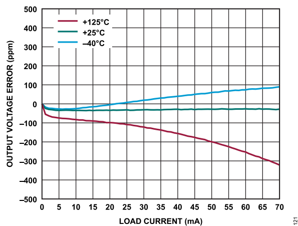
Figure 21. Output Voltage Error vs. Load Current
