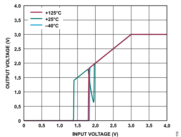
Figure 19. ADR3630 Output Voltage vs. Input Voltage
