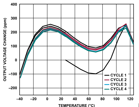
Figure 64. Change in Output Voltage over Four Full Temperature Cycle
