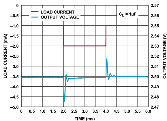
Figure 29. ADR3625 Load Transient Response (Source)
