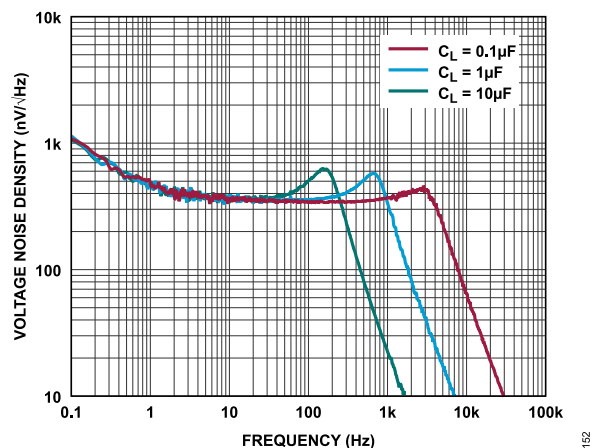
Figure 52. ADR3630 Voltage Noise Density
