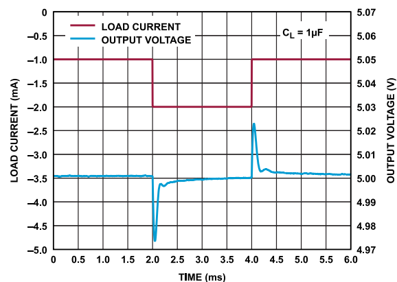
Figure 30. ADR3650 Load Transient Response (Source)
