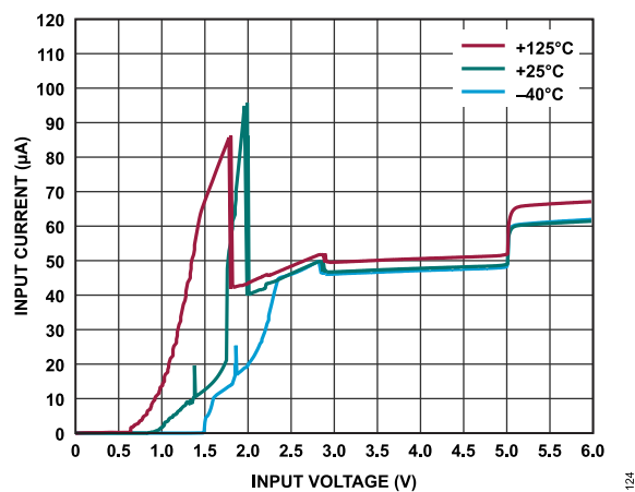
Figure 24. ADR3650 Input Current vs. Input Voltage
