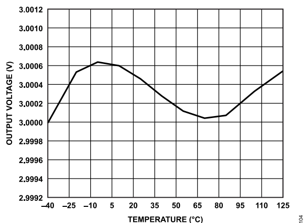
Figure 4. ADR3630 Output Voltage vs. Temperature
