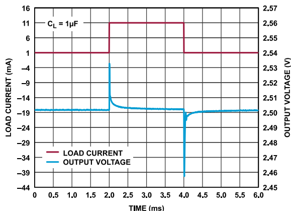
Figure 72. ADR3625 10 mA Sinking Response
