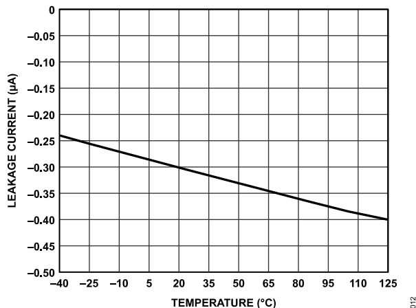
Figure 14. Leakage Current (Shutdown) vs. Temperature
