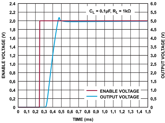
Figure 37. ADR3650 Start-Up Response (Enable)
