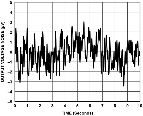
Figure 42. ADR3625 Voltage Noise (0.1 Hz to 10 Hz)
