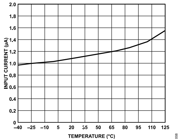
Figure 12. Input Current (Shutdown) vs. Temperature
