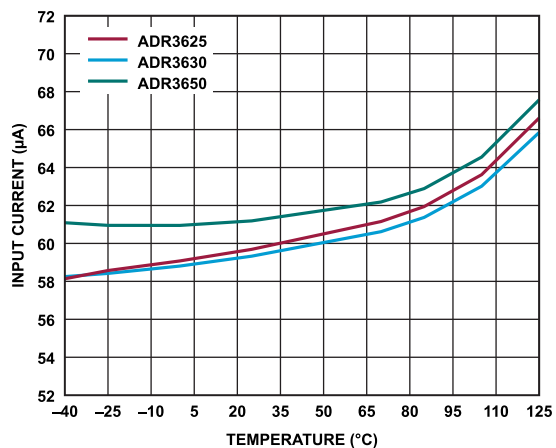
Figure 11. Input Current vs. Temperature
