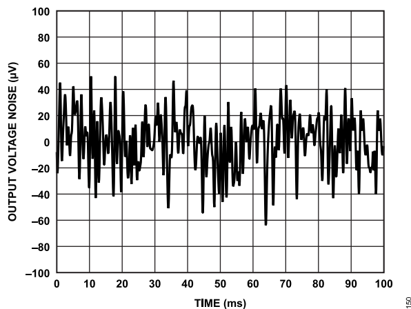
Figure 50. ADR3650 Output Voltage Noise (10 Hz to 1 kHz)
