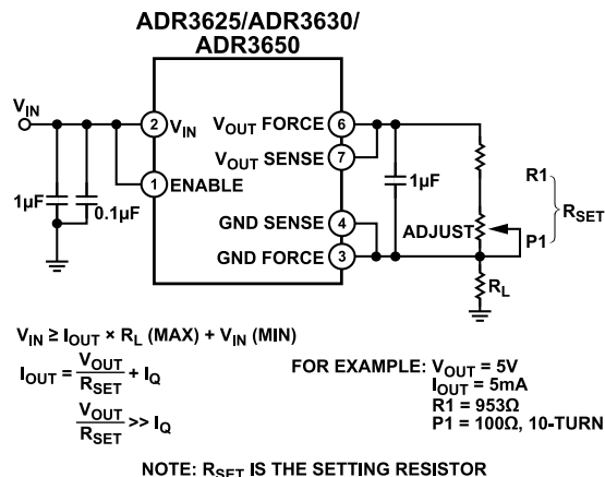
Figure 80. Constant Current
