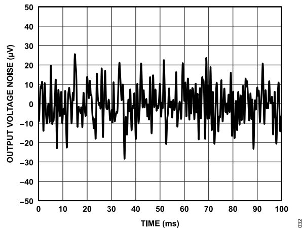
Figure 48. ADR3625 Output Voltage Noise (10 Hz to 1 kHz)
