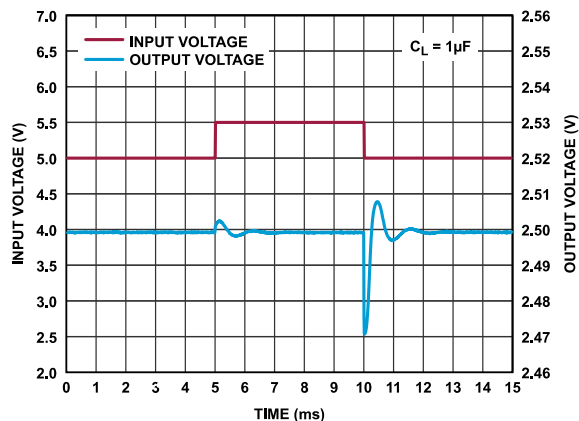
Figure 27. ADR3625 Line Transient Response
