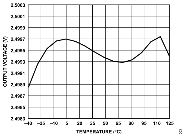
Figure 3. ADR3625 Output Voltage vs. Temperature
