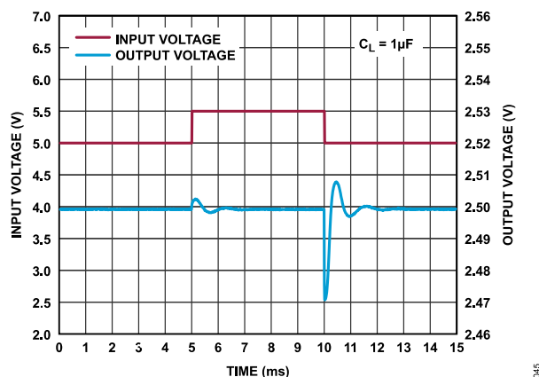
Figure 74. ADR3625 Output Response with a 500 mV Step on V_{IN}
