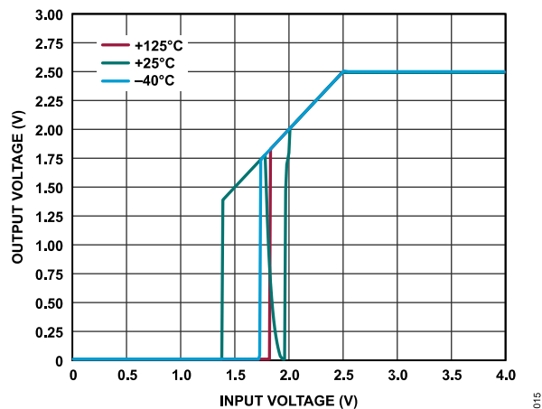
Figure 18. ADR3625 Output Voltage vs. Input Voltage
