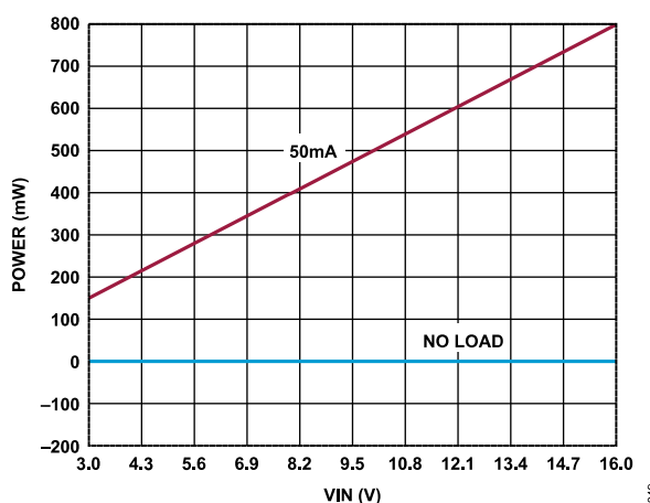
Figure 62. ADR3625 Typical Power Dissipation
