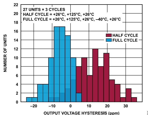
Figure 65. Output Voltage Hysteresis Histogram (-40°C to +125°C)
