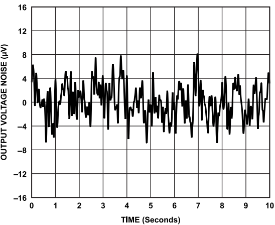
Figure 44. ADR3650 Voltage Noise (0.1 to 10 Hz)
