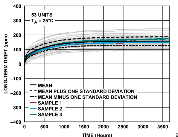
Figure 63. Long-Term Drift
