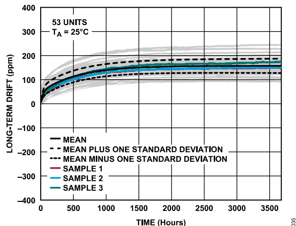
Figure 55. Long-Term Drift
