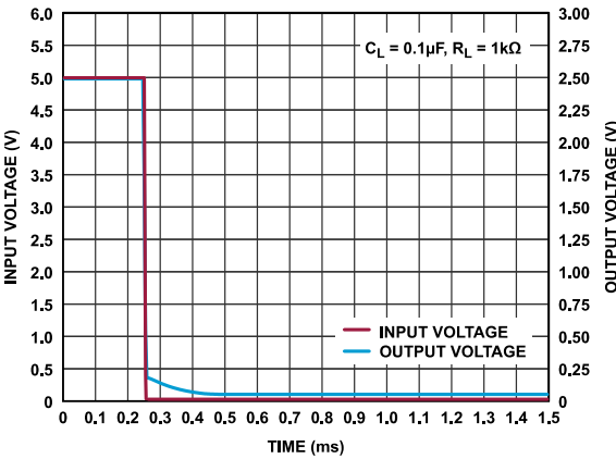
Figure 38. ADR3625 Shutdown Response (Input)
