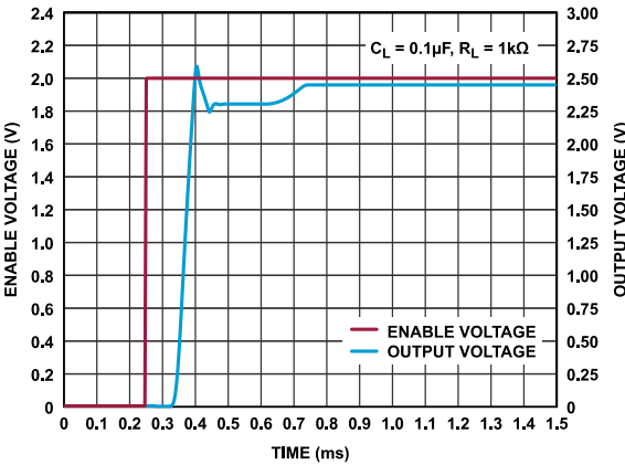
Figure 36. ADR3625 Start-Up Response (Enable)
