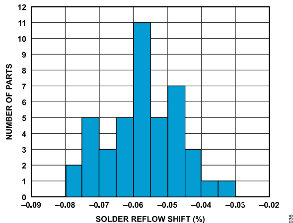
Figure 56. Solder Heat Reflow Shift Histogram
