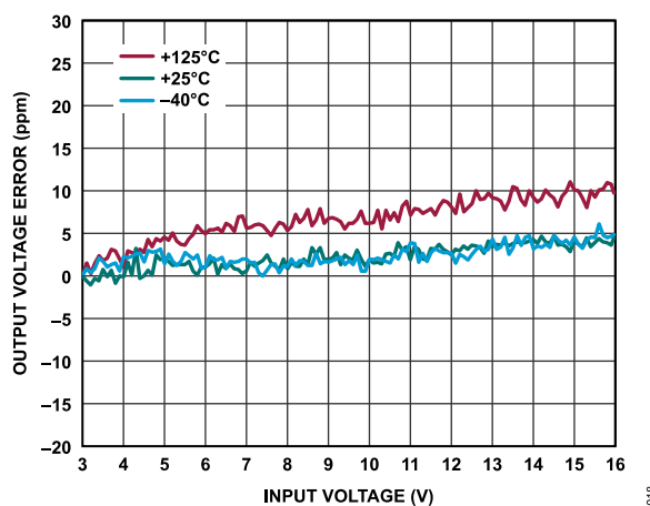
Figure 25. ADR3625 Output Voltage Error vs. Input Voltage
