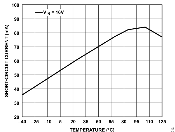
Figure 16. Short-Circuit Current (Sink) vs. Temperature
