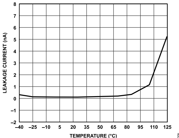
Figure 13. Leakage Current vs. Temperature
