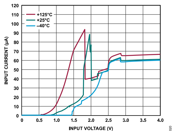
Figure 22. ADR3625 Input Current vs. Input Voltage
