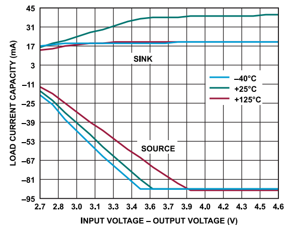
Figure 17. Load Current Capacity vs. Voltage Difference
