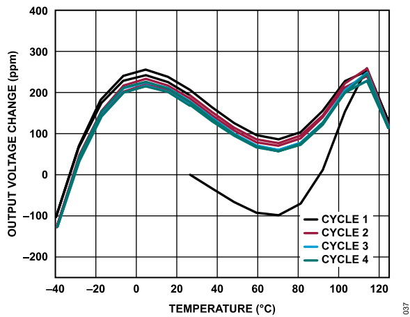
Figure 58. ADR3625 Hysteresis
