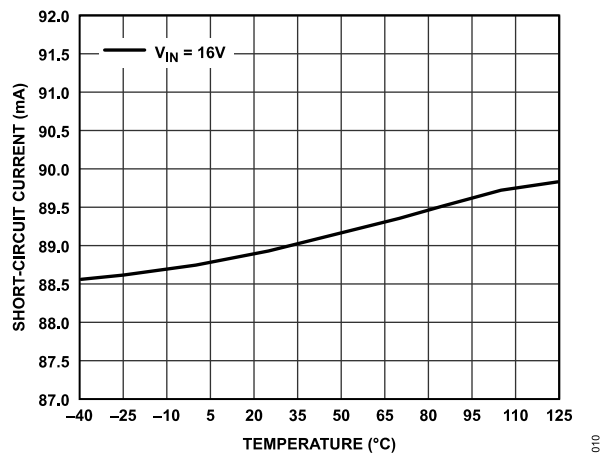
Figure 15. Short-Circuit Current (Source) vs. Temperature
