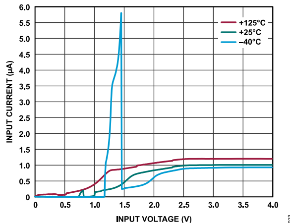
Figure 26. Input Current vs. Input Voltage (Shutdown)
