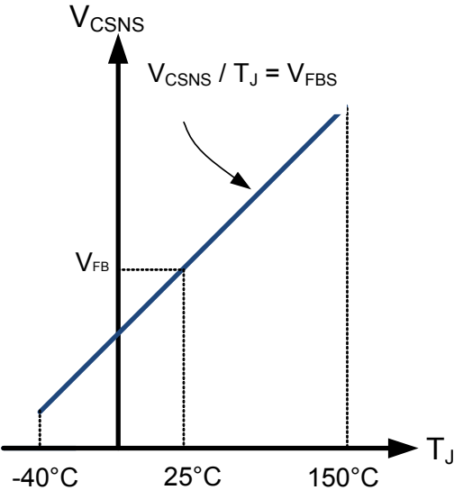
Figure 29. Temperature Reporting
