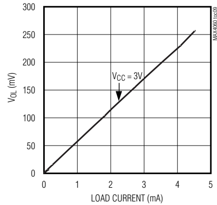
OUTPUT-VOLTAGE LOW vs. LOAD CURRENT
