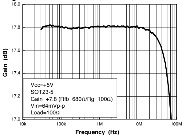
Figure 18. Gain flatness, G=+7.8 , SOT23-5L
