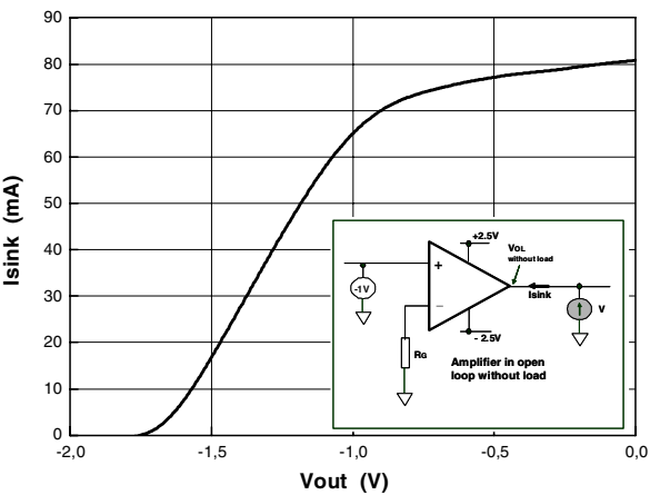
Figure 40. I sink
