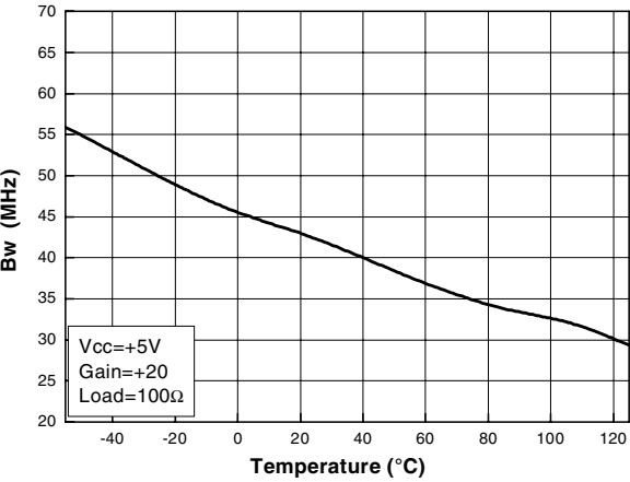
Figure 38. Bandwidth vs. temperature
