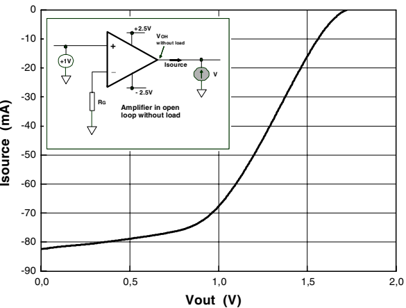
Figure 42. I source
