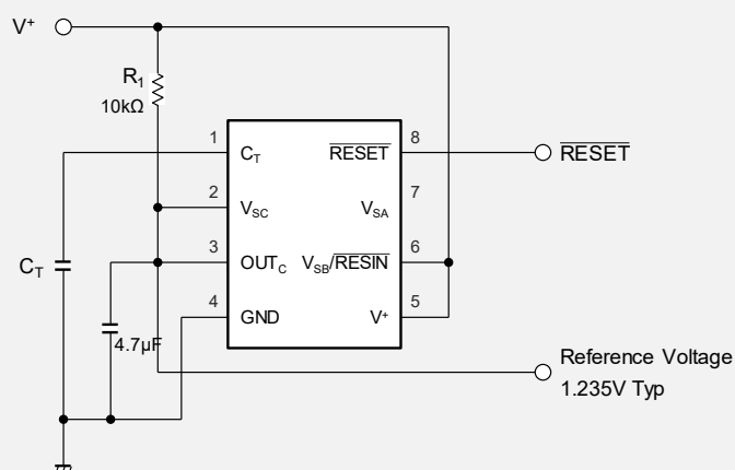
Fig. 13 Reference Voltage output and Voltage drop monitoring (e.g. 1.235V output, 5V monitoring)
