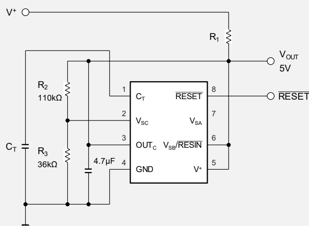
Fig. 12-2 Reference Voltage output and Voltage drop monitoring (e.g. 5V output, 5V monitoring)
