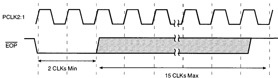
Figure 42. \overline{DREQ} and \overline{DACK} Functional Timing
