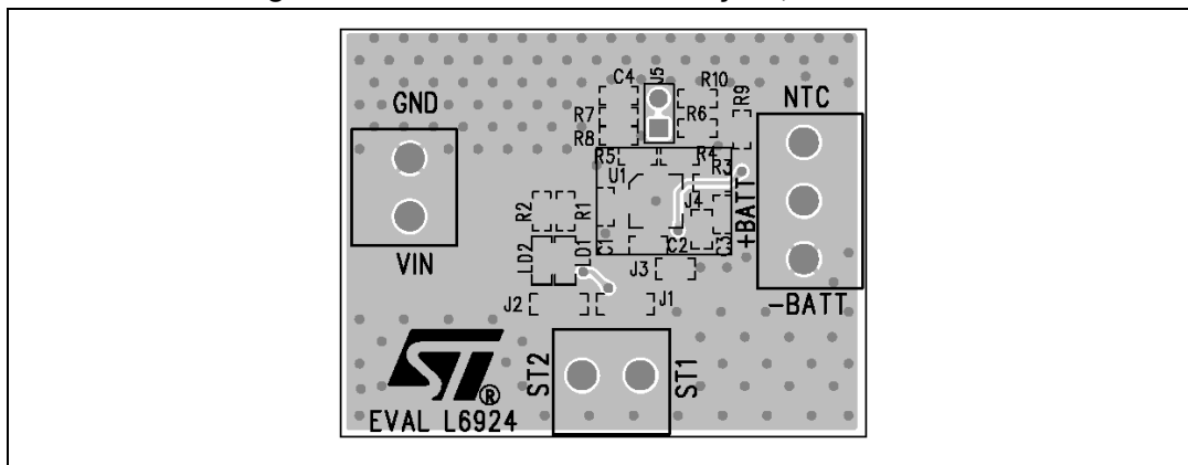
Figure 29. Demonstration board layout, bottom side
