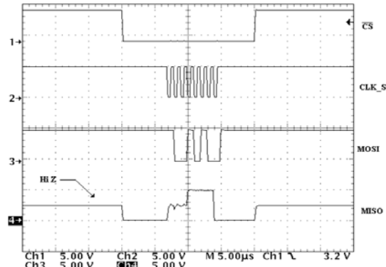
Figure 14. Programming Sequence
