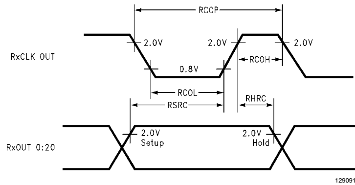
FIGURE 7. D590CR216 (Receiver) Setup/Hold and High/Low Times
