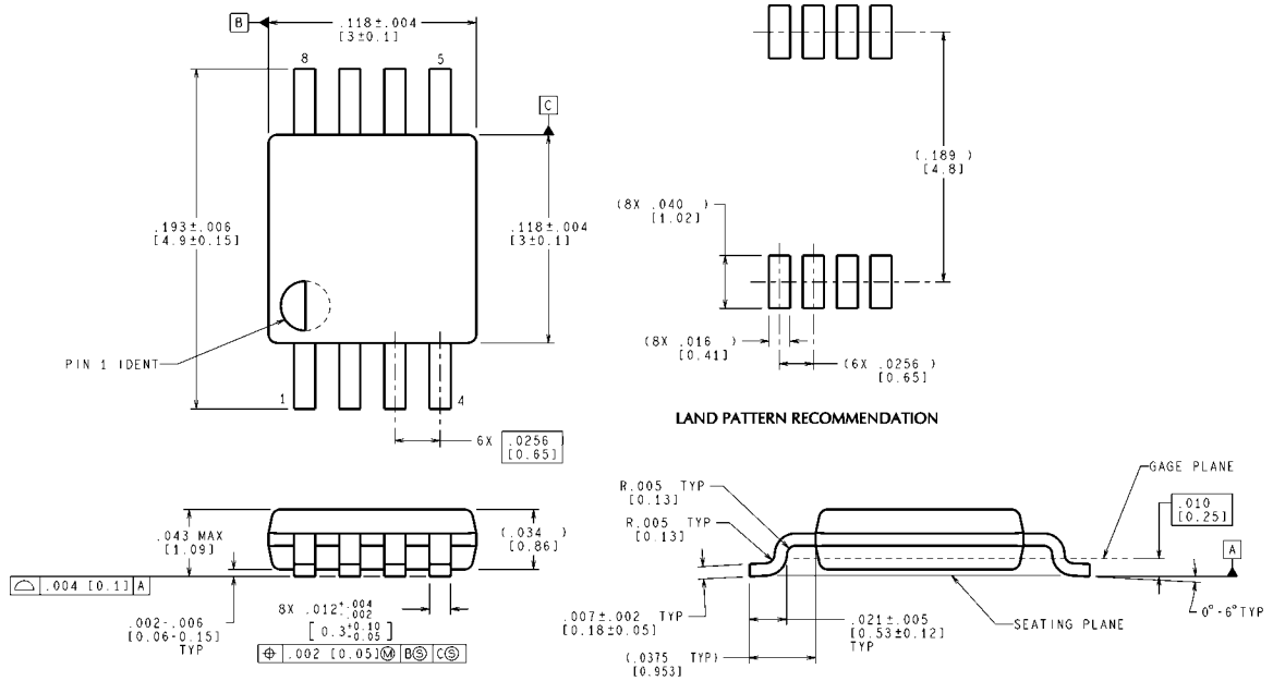
MSOP-8 Package NS Package Number MUA08A
