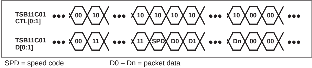
Figure 8. Receive Timing
