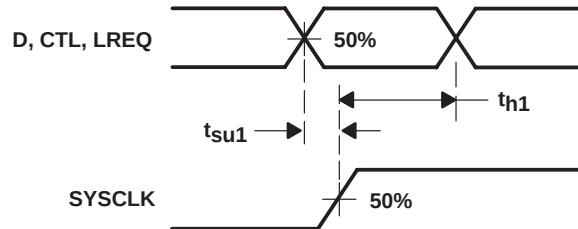
Figure 1. D, CTL Output Delay Relative to SYSCLK Waveforms
