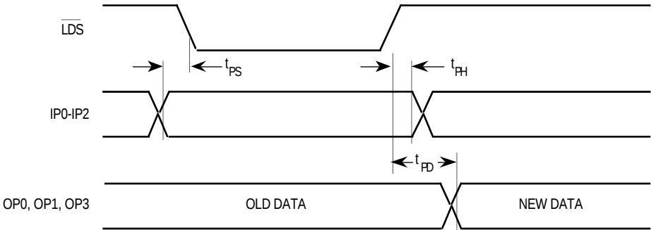
Figure 8-13. Port Timing
