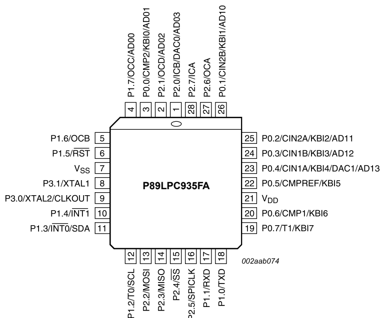
Fig 4. P89LPC935 PLCC28 pin configuration
