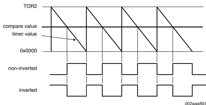
Fig 10. Asymmetrical PWM, down-counting mode
