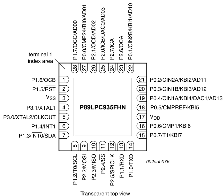
Fig 5. P89LPC935 HVQFN28 pin configuration
