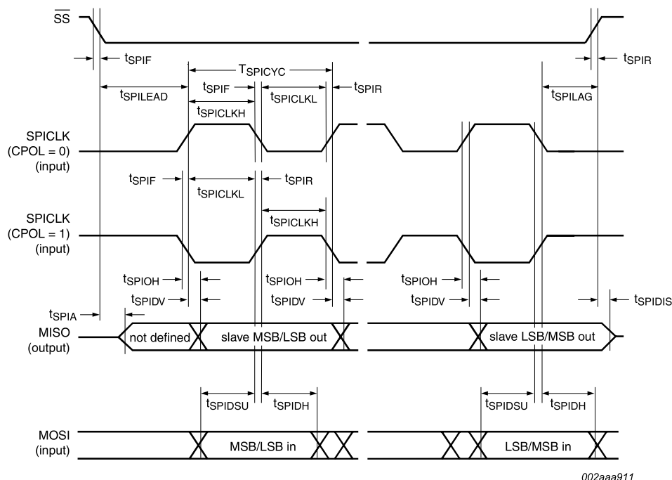
Fig 30. SPI slave timing (CPHA = 1)
