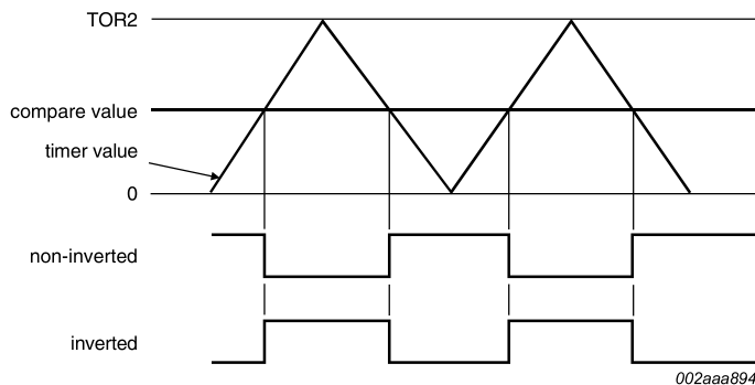
Fig 11. Symmetrical PWM
