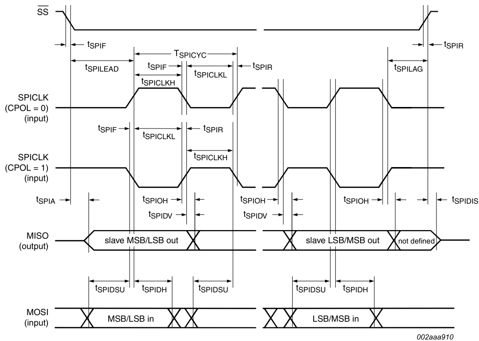
Fig 29. SPI slave timing (CPHA = 0)
