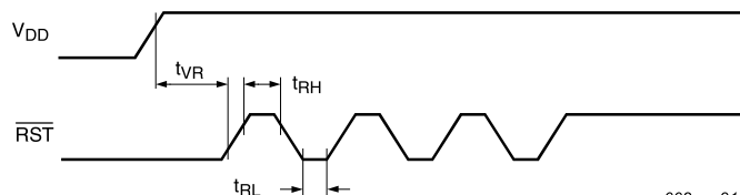
Fig 31. ISP entry timing
