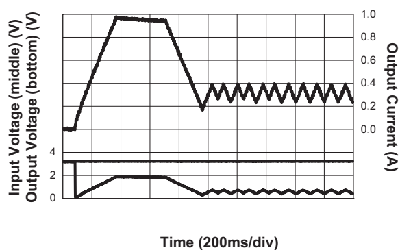
Short Circuit with 5Ω Series Impedance ( V_{IN} = 3.3V )
