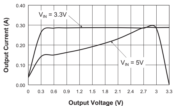
Output Current vs. Output Voltage ( R_{SETU} = 383k\Omega , 25^\circ\text{C} )
