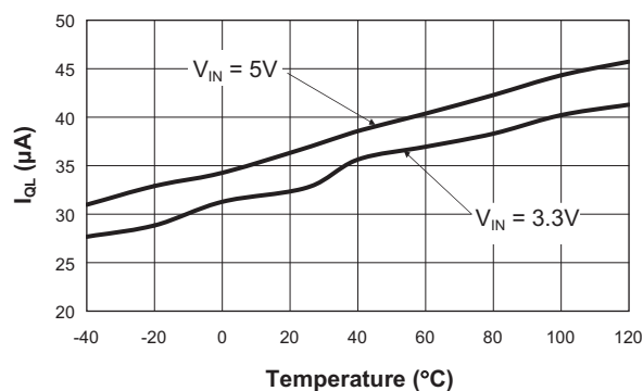
Quiescent Current I_{QL} vs. Temperature ( ENLB = 0V ; ENUB = V_{CC} ; V_{OUT} = \text{Open} )
