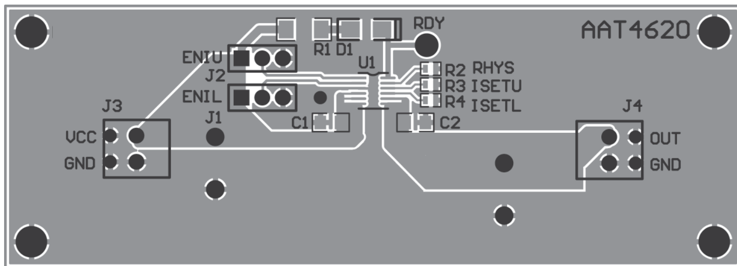
Figure 3: AAT4620 Evaluation Board PCB Top Side.
