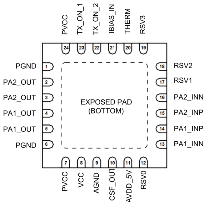
Figure 3. Pin connections
