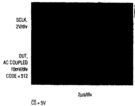
DIGITAL FEEDTHROUGH ( f_{SCLK} = 100kHz )
