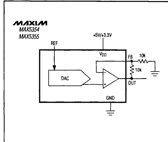
Figure 9. Unipolar Rail-to-Rail Output Circuit
