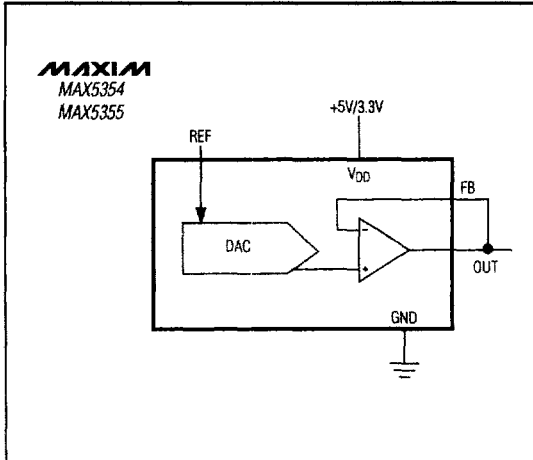
Figure 8. Unipolar Output Circuit
