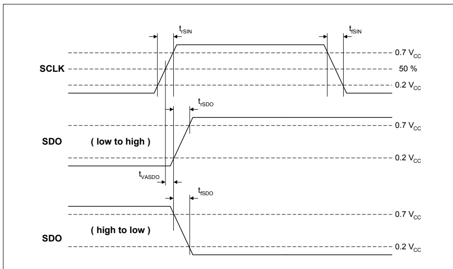
Figure 10 DO Valid Data Delay Time and Valid Time
