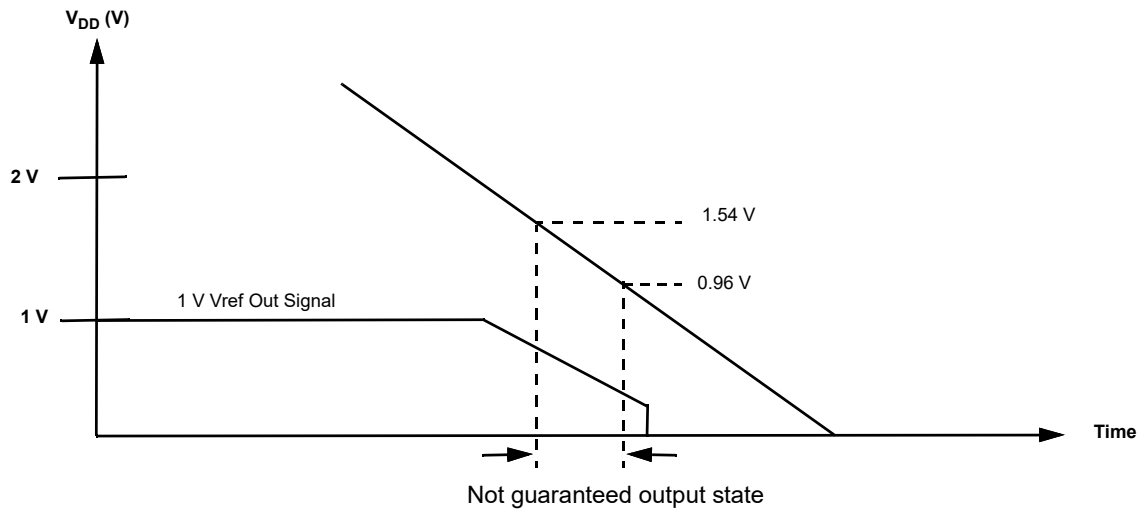
Figure 234: Power-Down
