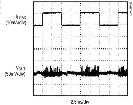
LOAD-TRANSIENT RESPONSE
