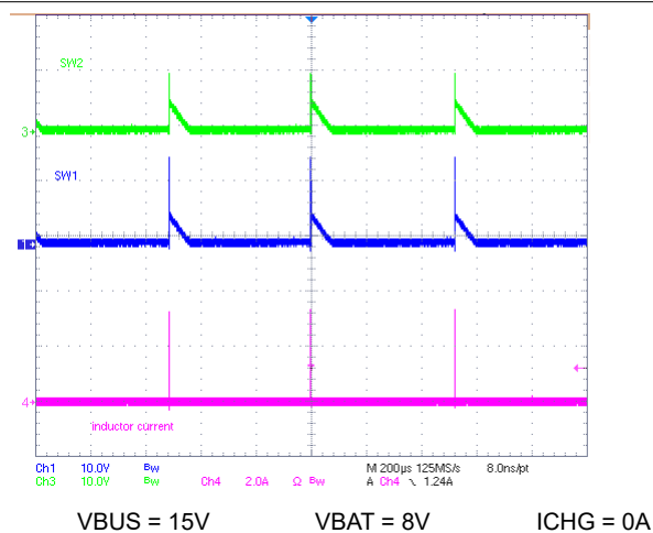
Figure 9-4. Buck Mode PFM without OOA
