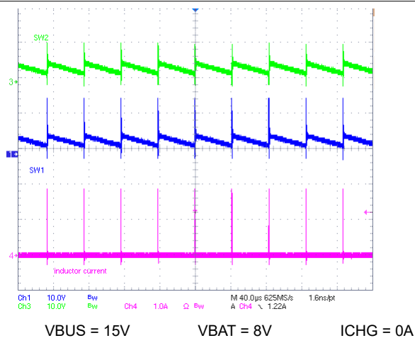
Figure 9-3. Buck Mode PFM with OOA
