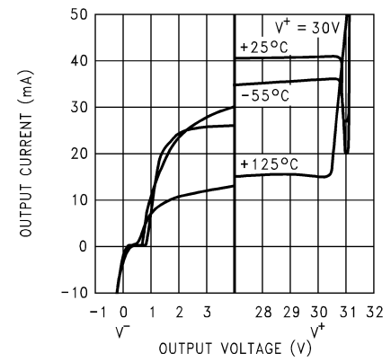
Output Sink Current vs. Output Voltage and Temp.
