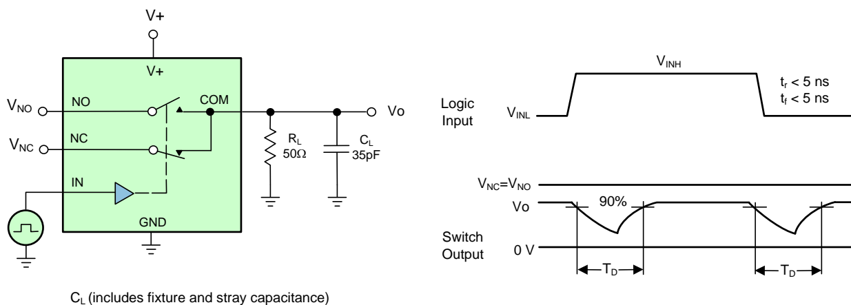
Figure 2 — Break-Before-Make Interval
