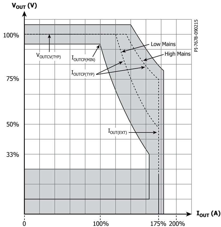
Figure 15. Typical LNK4214D and LNK4215D CP Output Characteristic Achieved.
