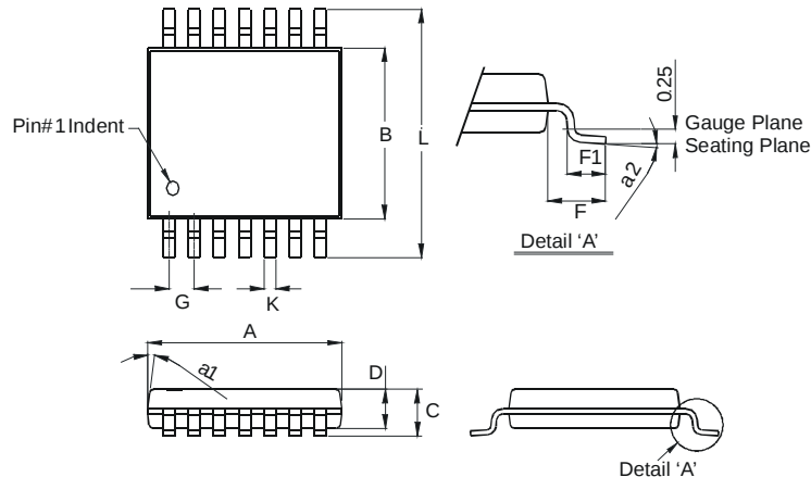
TSSOP-14
