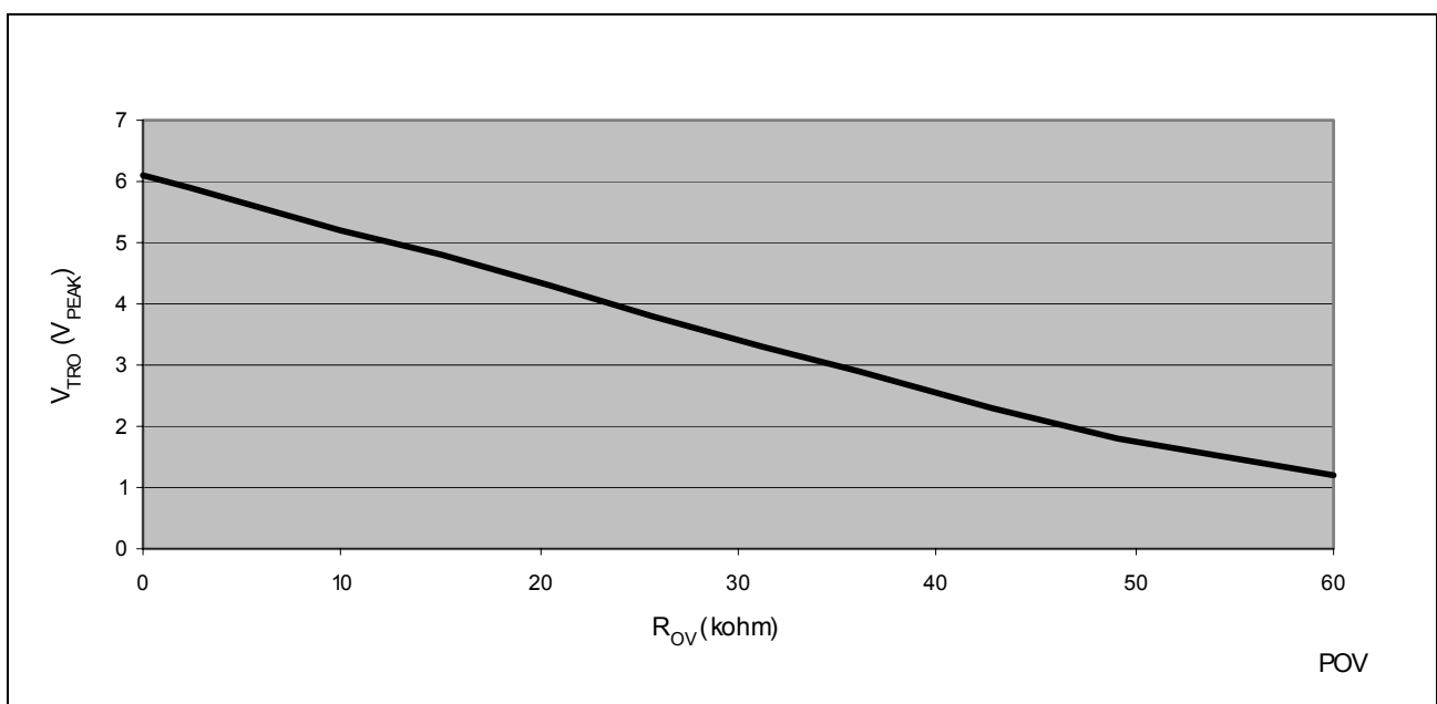
Figure 13 Programmable Overhead Voltage (POV). R_{\text{L}} = 600 \Omega or Infinite
