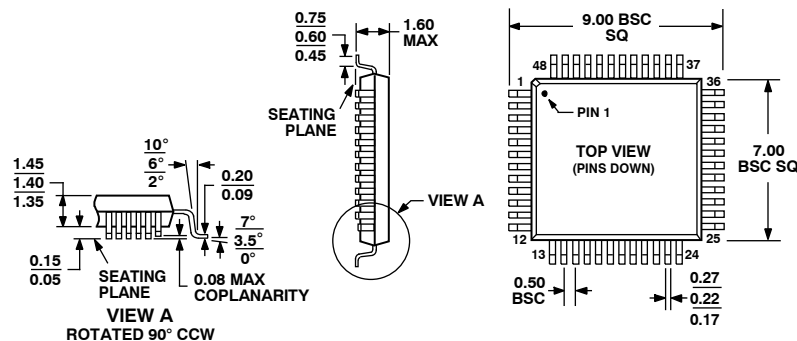
Figure 63. 48-Lead Thin Plastic Quad Flat Package [LQFP] 7 mm x 7 mm x 1.4 mm Thick (ST-48) Dimensions shown in millimeters
