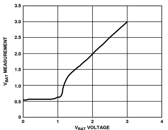
Figure 15. V_{BAT} Measurement vs. Voltage
