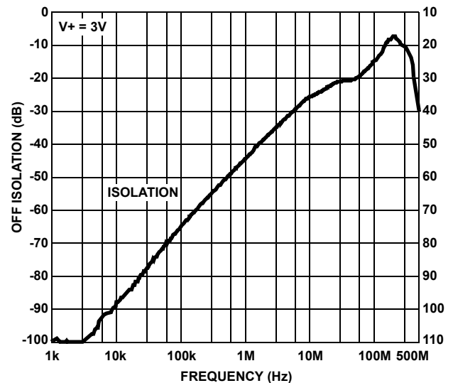
FIGURE 17. OFF ISOLATION
