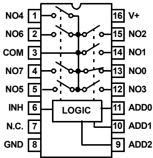
ISL84781 (TSSOP) TOP VIEW
