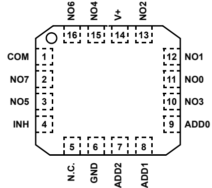
ISL43L680 (3x3 QFN) TOP VIEW
