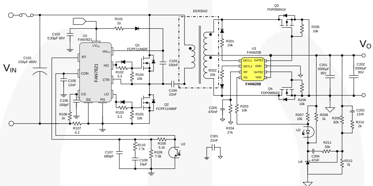
Figure 44. Application Circuit
