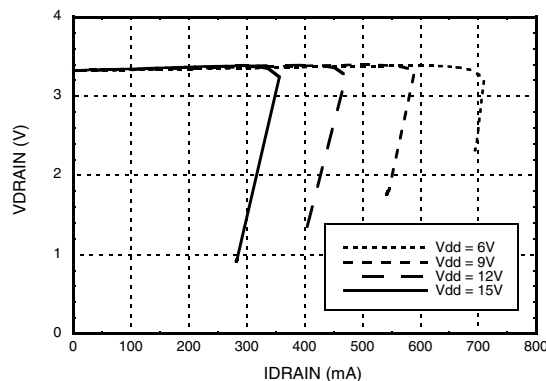
Power Foldback VDRAIN vs. IDRAIN over V DD
