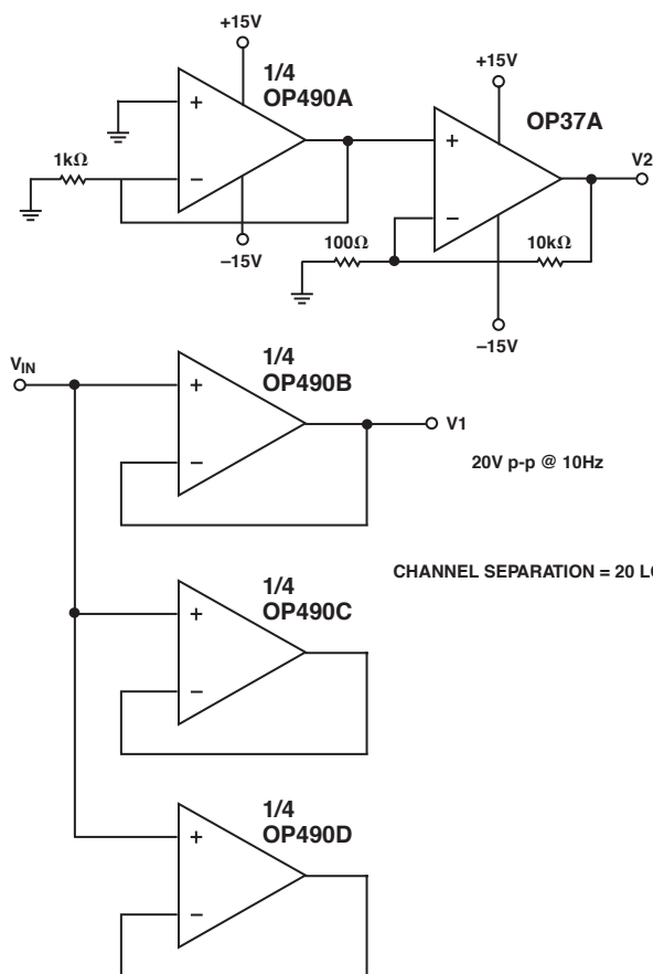
Figure 3. Channel Separation Test Circuit
