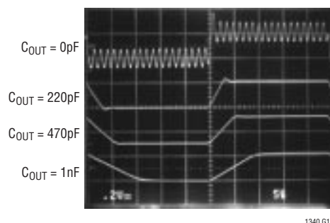
Small-Signal Response
