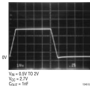
Large-Signal Response
