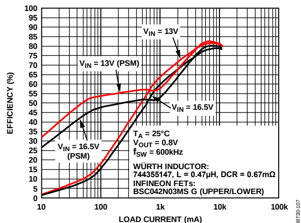
Figure 7. Efficiency—600 kHz, V_{OUT} = 0.8\text{ V}
