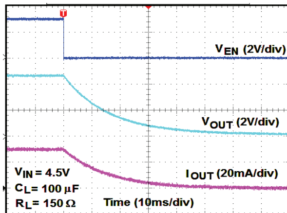
Fig. 25 - Turn-Off Time, SiP32458
