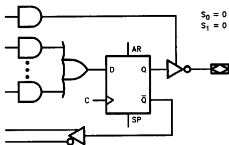
FIGURE 3-1. Registered/Active Low
