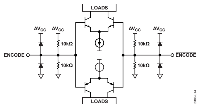
Figure 15. ENCODE Inputs
