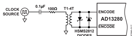
Figure 17. Crystal Clock Oscillator—Differential Encode
