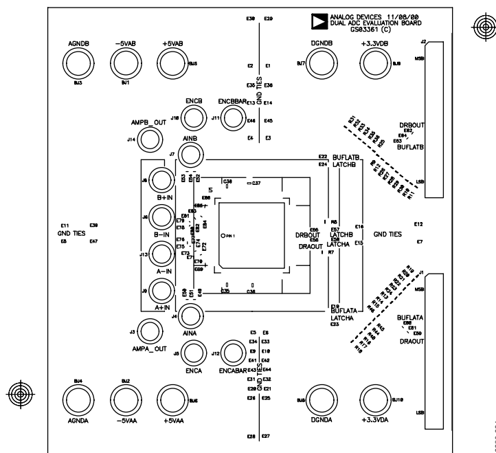
Figure 24. Top Silk
