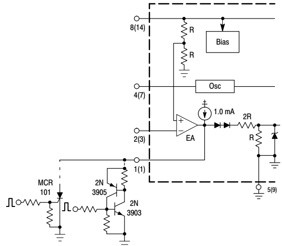
The MCR101 SCR must be selected for a holding of < 0.5 \text{ mA} @ T_{A(\min)} . The simple two transistor circuit can be used in place of the SCR as shown. All resistors are 10 k.
