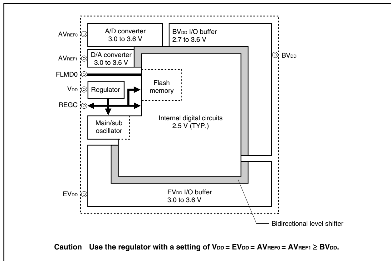
Figure 25-1. Regulator
