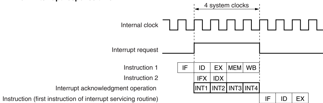
Figure 19-15. Pipeline Operation at Interrupt Request Signal Acknowledgment (Outline)
