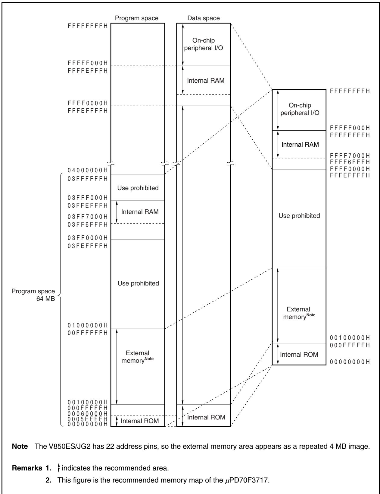
Figure 3-15. Recommended Memory Map
