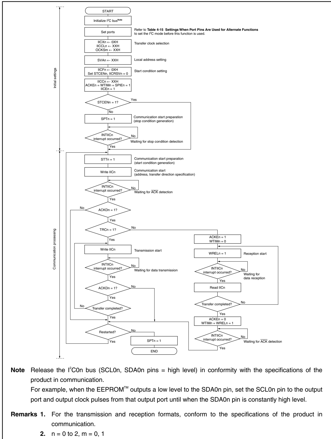
Figure 17-18. Master Operation in Single Master System
