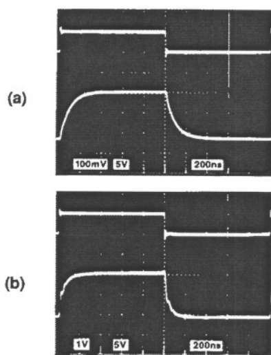
FIGURE 13: Pulse response of the AGC amplifier at (a) low level input signal, and (b) large input signal.
