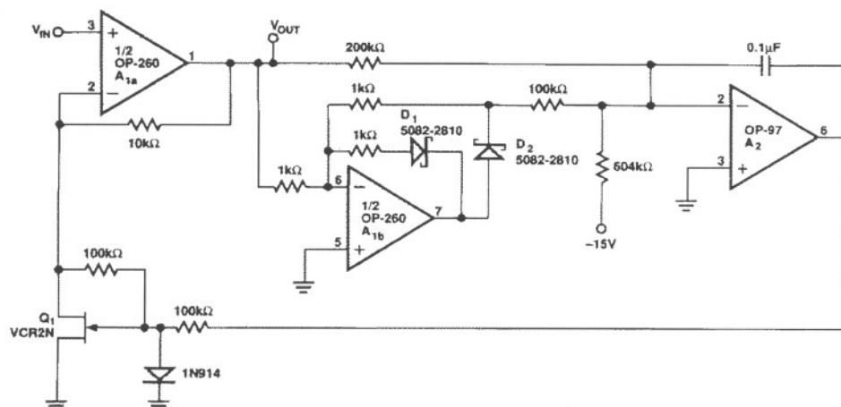
FIGURE 12: The OP-260 eliminates the problem of variable bandwidth in AGC amplifiers using voltage feedback op amps.
