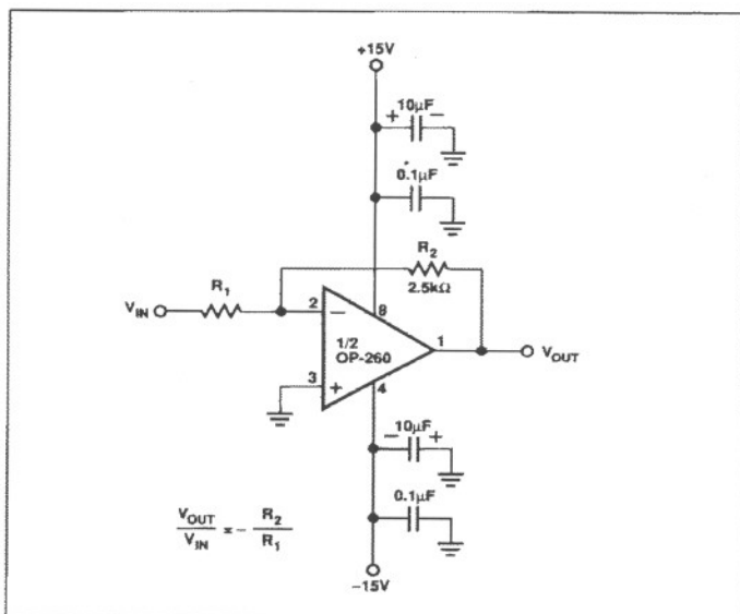
FIGURE 10: The OP-260 as an inverting amplifier.
