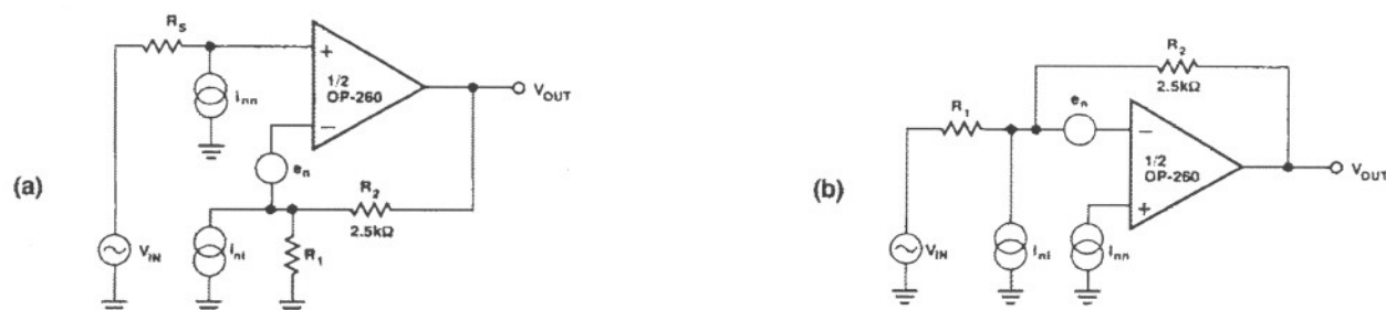
FIGURE 7: Simplified noise models for the OP-260 in noninverting (a) and inverting (b) gain.
