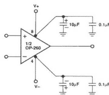
FIGURE 8: Proper power supplying bypassing is required to obtain optimum performance with the OP-260.
