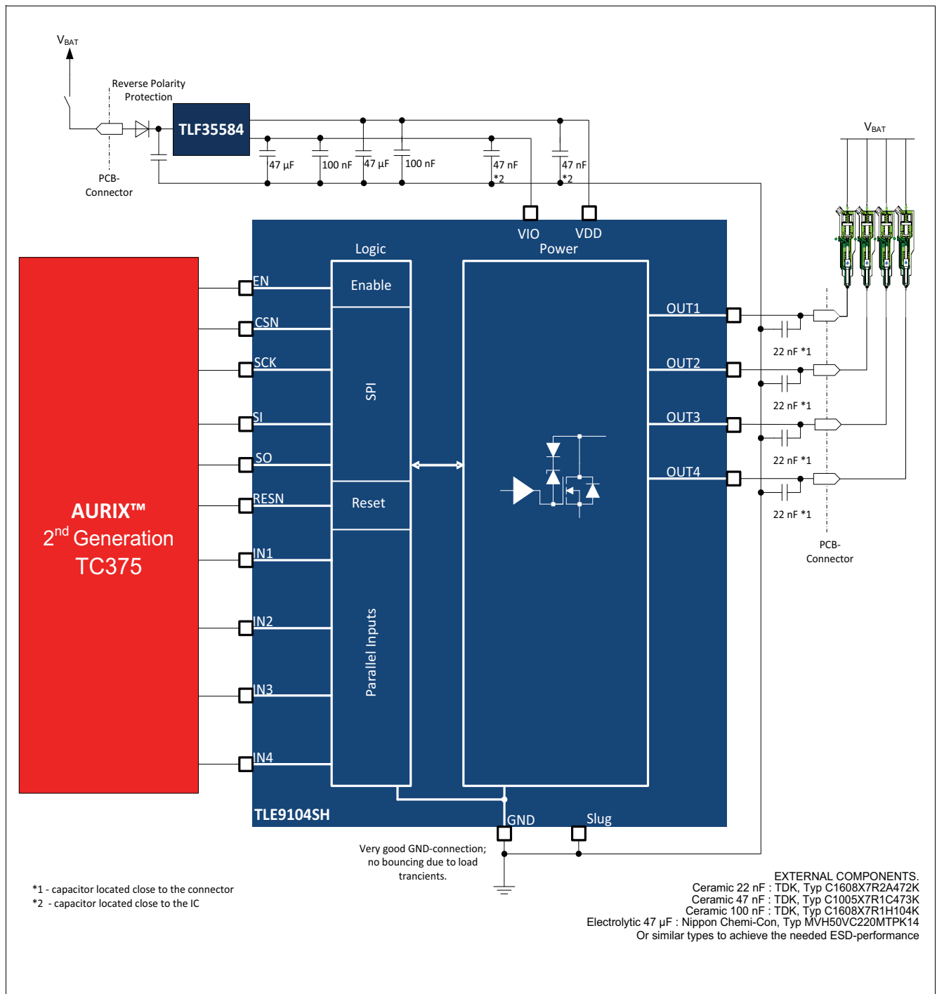
Figure 8-1 Multi port injection application diagram
