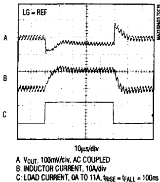
MAX1624 LOAD-TRANSIENT RESPONSE (WITH GLITCHCATCHER) (3.5V)
