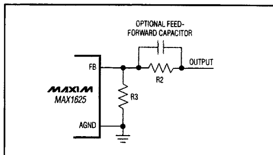
Figure 9. MAX1625 Optional Feed-Forward Compensation Capacitors
