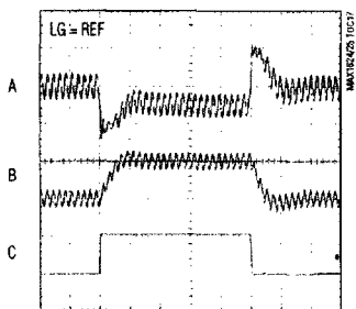
MAX1624 LOAD-TRANSIENT RESPONSE (WITH GLITCHCATCHER) (2.5V)
