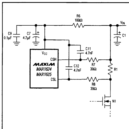
Figure 6. Current-Sense Filter
