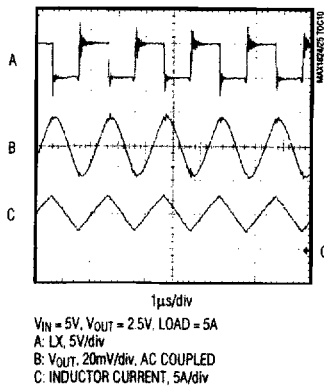
MAX1624 SWITCHING WAVEFORMS
