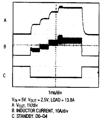
MAX1624 STARTUP AND STANDBY RESPONSE
