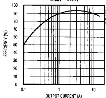
MAX1624 EFFICIENCY vs. OUTPUT CURRENT ( V_{OUT} = 3.5\text{V} )
