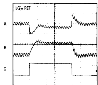
MAX1624 LOAD-TRANSIENT RESPONSE (WITHOUT GLITCHCATCHER) (3.5V)
