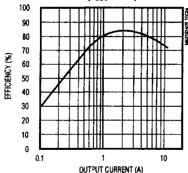
MAX1624 EFFICIENCY vs. OUTPUT CURRENT ( V_{OUT} = 1.1\text{V} )
