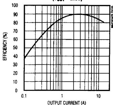
MAX1624 EFFICIENCY vs. OUTPUT CURRENT ( V_{OUT} = 2.5\text{V} )
