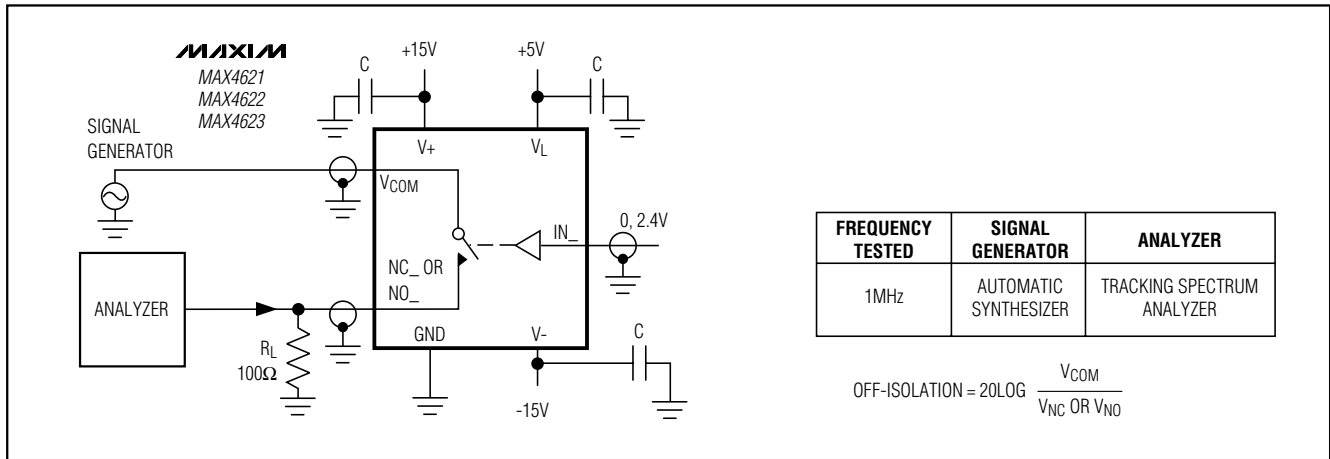
Figure 5. Off-Isolation
