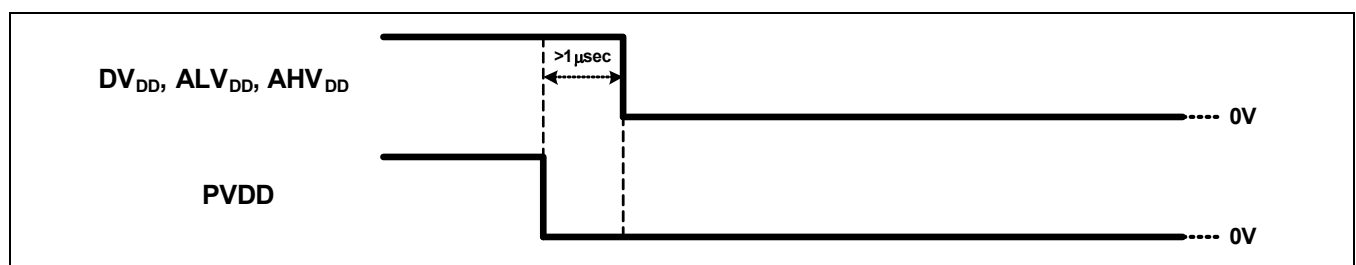
Figure 3-4. Power-Down
