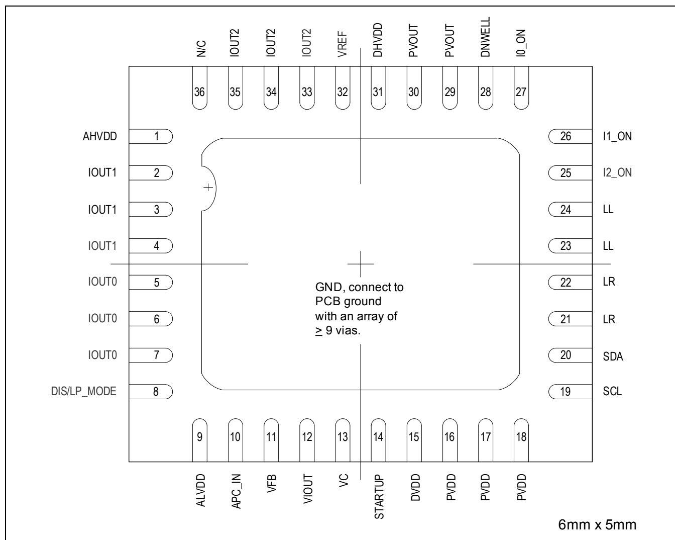
Figure 2-1. M08889 Pinout
