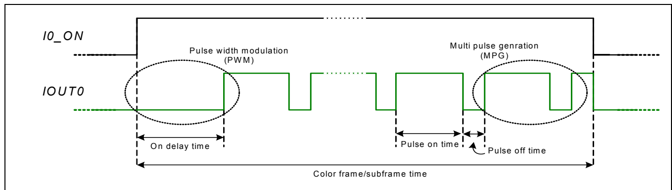
Figure 3-1. Example of PWM and MPG Timers
