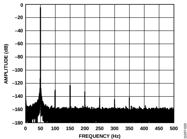
Figure 15. 50 Hz Input Tone, -6\text{ dBFS} Input FFT ( V_{REF} = 2.5\text{ V} , Output Data Rate = 1 kSPS)
