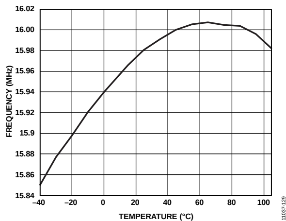
Figure 29. Internal Oscillator Frequency vs. Temperature
