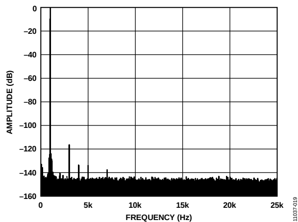
Figure 14. 1 kHz Input Tone, -0.5\text{ dBFS} Input FFT ( V_{REF} = 2.5\text{ V} , Output Data Rate = 50 kSPS)
