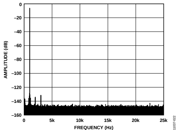
Figure 16. 1 kHz Input Tone, -6\text{ dBFS} Input FFT ( V_{REF} = 2.5\text{ V} , Output Data Rate = 50 kSPS)
