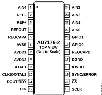
Figure 4. Pin Configuration
