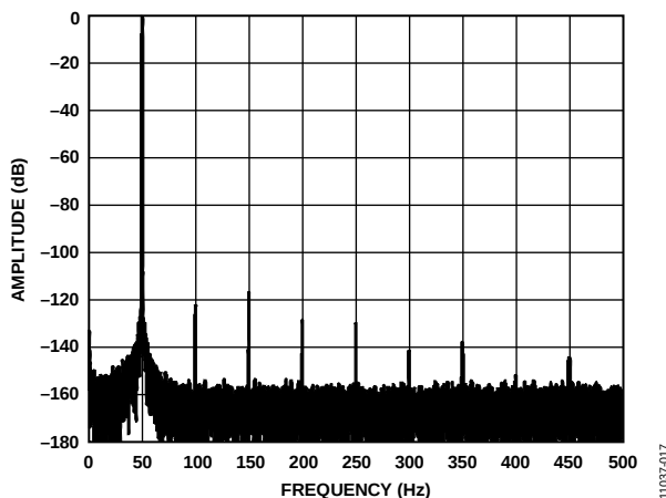
Figure 13. 50 Hz Input Tone, -0.5\text{ dBFS} Input FFT ( V_{REF} = 2.5\text{ V} , Output Data Rate = 1 kSPS)
