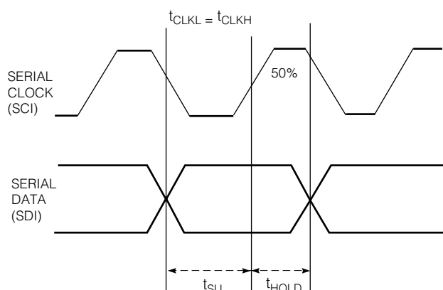
Fig. 7 Waveforms
