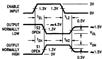
FIGURE 4. Enable and Disable Times (Notes 1, 2 and 3)
