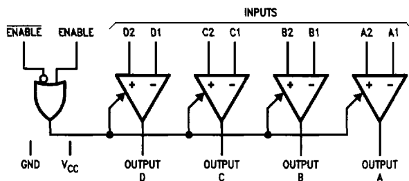
FIGURE 1. Logic Symbol
