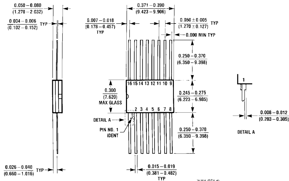
16-Lead Ceramic Flat Package (W) Order Number 54LS279FMB or DM54LS279W Package Number W16A
