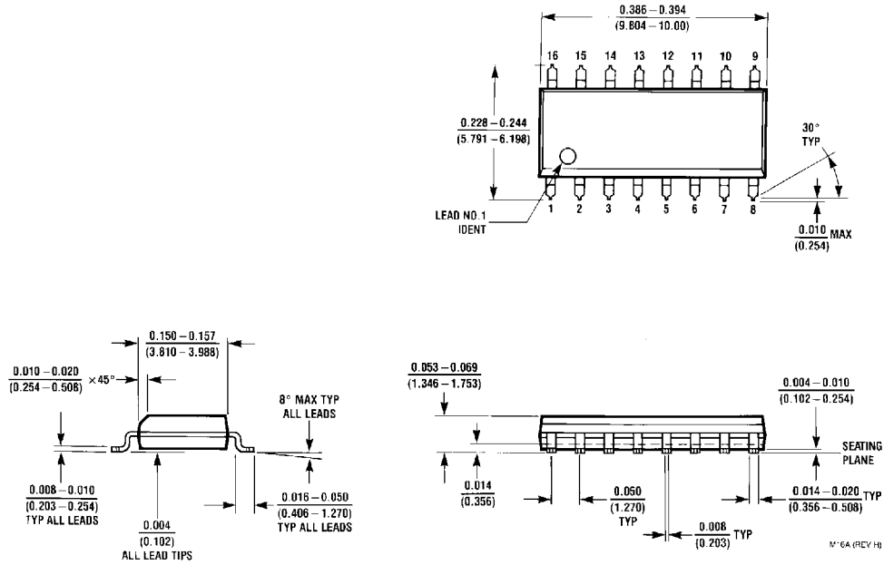
16-Lead Small Outline Molded Package (M) Order Number DM74LS279M Package Number M16A
